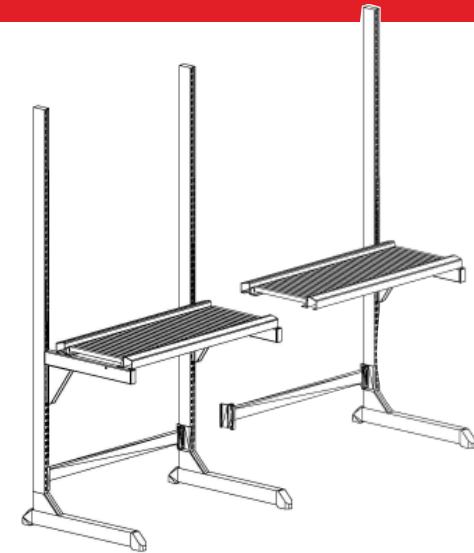
M36 Packing transfer start frame part no. 14-C12341181 M36 Packing transfer extension frame part no. 14-C12341182
